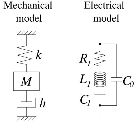
FIG. 3: (a) Mechanical model of the resonator as a damped oscillator and (b) electrical model which includes the motional (mechanical) equivalent series circuit in parallel with the electrical (capacitance between the electrodes separated by the quartz substrate) branch. See Tab. I for a summary of the equivalent quantities between the mechanical and electrical models.
