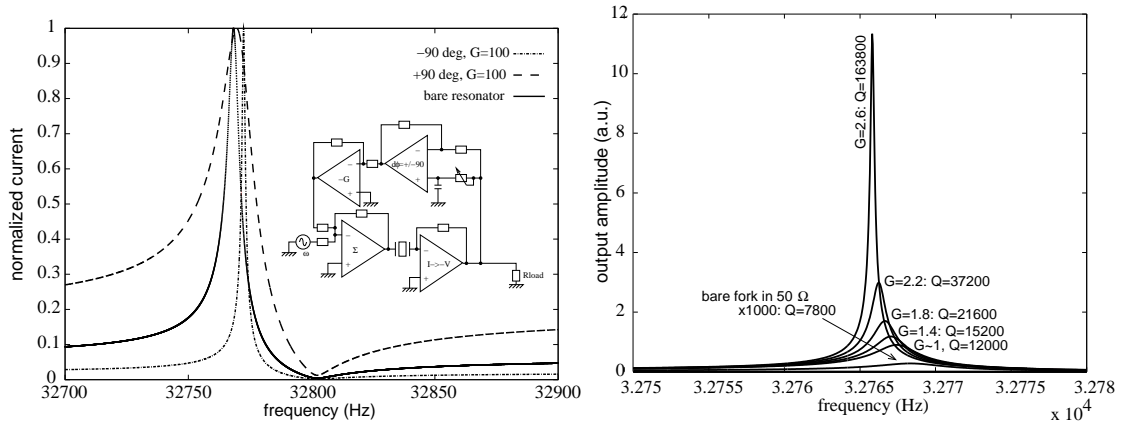
FIG. 8: (a) Circuit used for quality factor tuning and Spice simulation of the response as a function of amplifier gain. In addition to the quality factor enhancement, a frequency shift is associated with the phase of the feedback loop not being exactly equal to \pm 90^\circ . The normalized current is displayed for enhancing the visibility of the quality factor tuning. (b) Current output as a function of feedback loop gain leading to in-phase energy injection and current magnitude increase with the enhancement of the quality factor.
