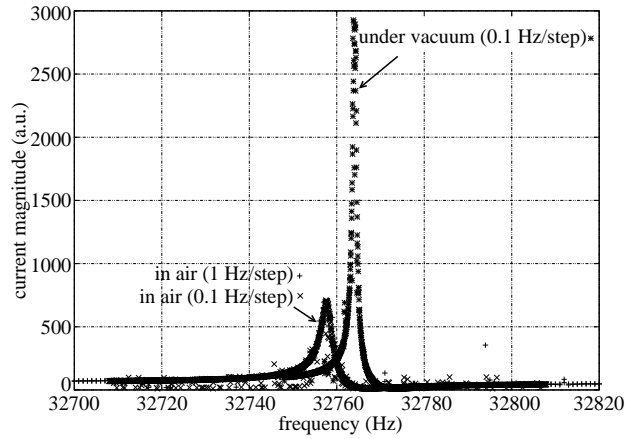
FIG. 4: Current measurement through packaged and opened tuning forks as a function of frequency. We observe first the resonance followed by the anti-resonance. Notice the signal drop and the peak widening due to viscous friction with air once the tuning fork is removed from its packaging.
