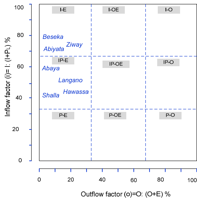
Figure 2. Classification of lakes by water balance criteria (inflow-outflow). (N.B: Lake Chamo was not considered in this result due to limited data availability).
