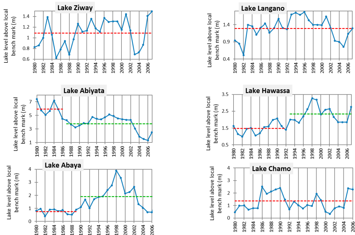
Figure 4. Long-term lake level plots of the six Ethiopian Rift Valley lakes. (N.B: (a) Analysis of regime shifts were done for the first six lakes using Pettit [34] homogeneity test. The red lines represent mean lake level before the regime shift ( \mu_1 ) and the green line after the regime shift ( \mu_2 ). (b) Lake Shalla and Beseka are not included in this result due to availability of time series data during the study).
