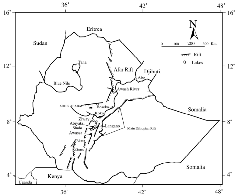
Figure 1. Relative locations of the Ethiopian rift-valley lakes (source: Alemayehu et al. [13]). (N.B: The original map does not show Lake Abaya and Chamo).
