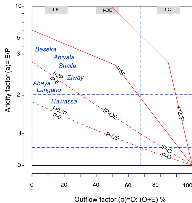
Figure 3. Classification of lakes by water balance criteria (aridity-outflow). (N.B: Lake Chamo was not considered in this result due to limited data availability).
