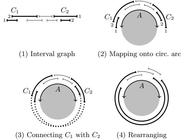
Fig. 2. Construction used in the proof of Lemma 1. Edges of the maximal cliques C_1 and C_2 are illustrated in bold. The colors of the intervals in C_1 and C_2 are indicated by the small numbers next to the intervals. In this example, a path of length 7 is mapped onto an arc A . Then pairs of vertices with the same color of the maximal cliques C_1 and C_2 are connected, which gives a cycle of length 5. Every coloring of C_5 requires 3 colors.
