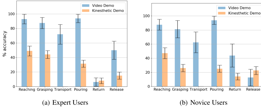
Figure 4: Reference frame detection accuracy for each action of the pouring task.
