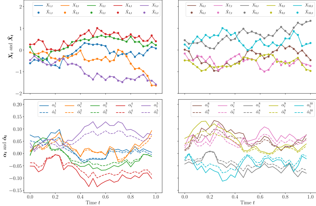
Figure 4: A sample path for each player of the general linear-exponential-quadratic game in Section 4.3 with N = 10 . Top: the optimal state process X_{i,t} (solid lines) and its approximation \hat{X}_{i,t} (circles) provided by the optimized neural networks, under the same realized path of Brownian motion. Bottom: comparisons of the strategies \alpha_t^i and \hat{\alpha}_t^i (dashed lines).
