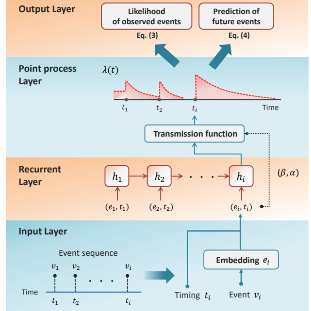
Figure 2: Schematic of the DDP Architecture.
