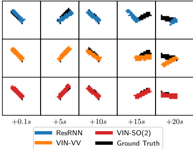
Figure 7: Reconstructions of the pendulum system from forecasts in latent space, using a step-size of 0.1s , up to 20s . The ground truth (black) is occluded by the model predictions, shown in color.
