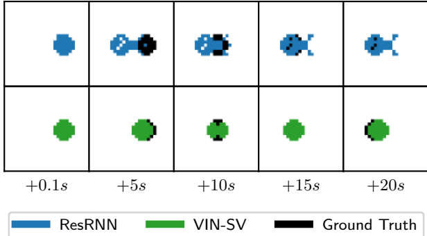
Figure 8: Reconstructions of the mass-spring system from forecasts in latent space, using a step-size of 0.1s , up to 20s . The ground truth (black) is occluded by the model predictions, shown in color. The mass oscillates left-and-right based on the initial tension in the spring (not rendered in images).
