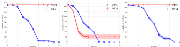
Figure 2: \ell_1 distance from ground truth ( Y axis) vs. number of iterations ( X axis). The line is the mean of 20 random trials and the shaded area shows the standard deviation. u is initialized from i.i.d. Bernoulli with mean \mu = 0.1, 0.5, 0.9 from the left to right.
