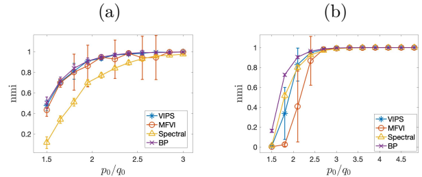
Figure 5: Comparison of VIPS, MFVI, Spectral and BP using error-bars from 20 random trials for n = 2000 , average degree 50, p_0/q_0 is changed on X axis. (a) \pi = 0.3 (b) K=3, B = (p-q)I + qJ . For BP, MFVI and VIPS, we use true parameters.
