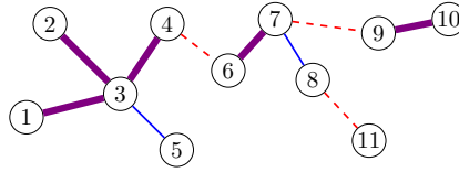
Figure 4: The graph G \vee G' with (G, G') of Figure 1. For the sake of readability, the two-colored edges of G \wedge G' are always drawn thick and purple.
