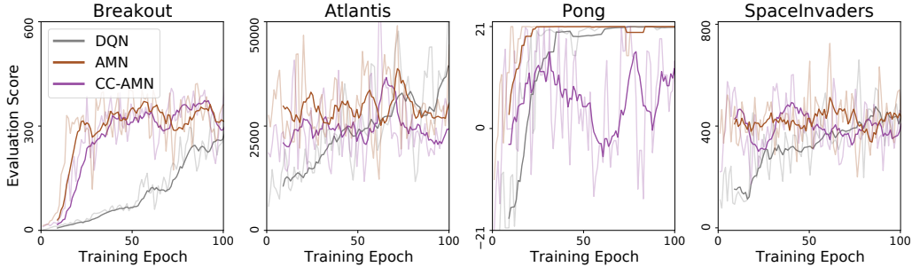
Figure 2: Training curves for the CC-AMN and AMN models, run on the simplified single-game objective. Solid lines reflect a moving average of the raw evaluation scores (faded lines). Each training epoch lasts 100 000 frames, with the evaluation scores being calculated from another 100 000 frames. While the actor-mimic models learn much faster than the DQN, the CC-AMN shows no improvement over the AMN model.
