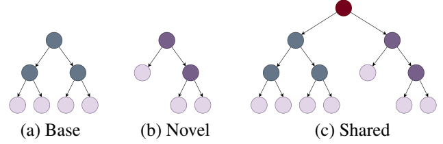
Figure 2. Tree expansion for novel classes: (a) A tree that was learned on the base classes; (b) On a novel session, we first build a tree from the novel classes representations; (c) Next we connect the trees using a shared root node.
