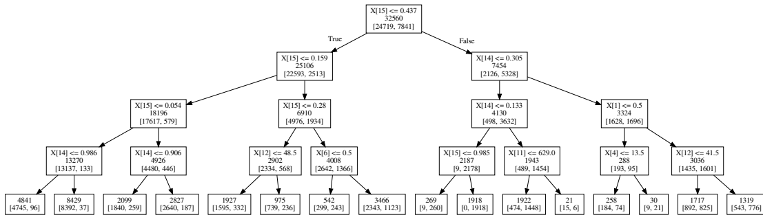
Figure S11. Adult dataset. Second-layer tree structure of depth 4 when the first-layer tree is of depth 9 (optimal depth). Raw features range from X[0] to X[13], X[14] and X[15] are the features built by the first-layer tree.
