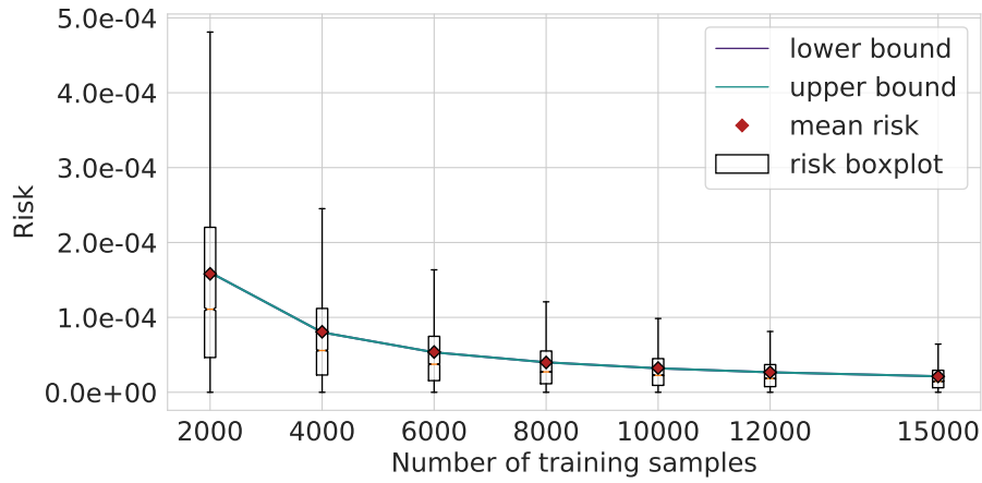
Figure S39. Illustration of the theoretical bounds for a shallow tree network of Proposition 4.2, for a chessboard with parameters k^* = 4 , N_B = 2^{k^* - 1} and p = 0.8 . The first-layer tree is of depth k = 4 . We draw a sample of size n (x-axis), and a single tree r_{k,0,n} is fitted for which the theoretical risk is evaluated. Each boxplot is built out of 20 000 repetitions. The outliers are not shown for the sake of presentation. Note that in such a case, the theoretical lower bound is constant and equal to the bias term. Note that the lower bound and the upper bound are merged.
