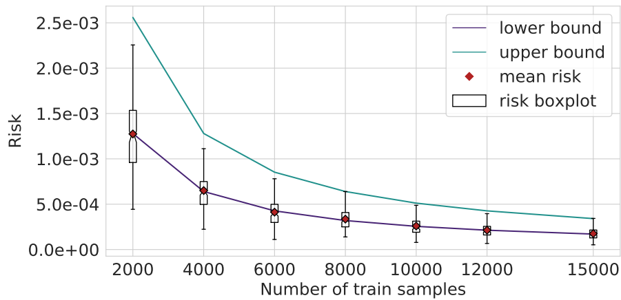
Figure S36. Illustration of the theoretical bounds for a single tree of Proposition 4 1. for a chessboard with parameters k^* = 4 , N_B = 2^{k^*-1} and p = 0.8 . The single tree is of depth k = 4 . We draw a sample of size n (x-axis), and a single tree r_{k,0,n} is fitted for which the theoretical risk is evaluated. Each boxplot is built out of 20 000 repetitions. The outliers are not shown for the sake of presentation.
