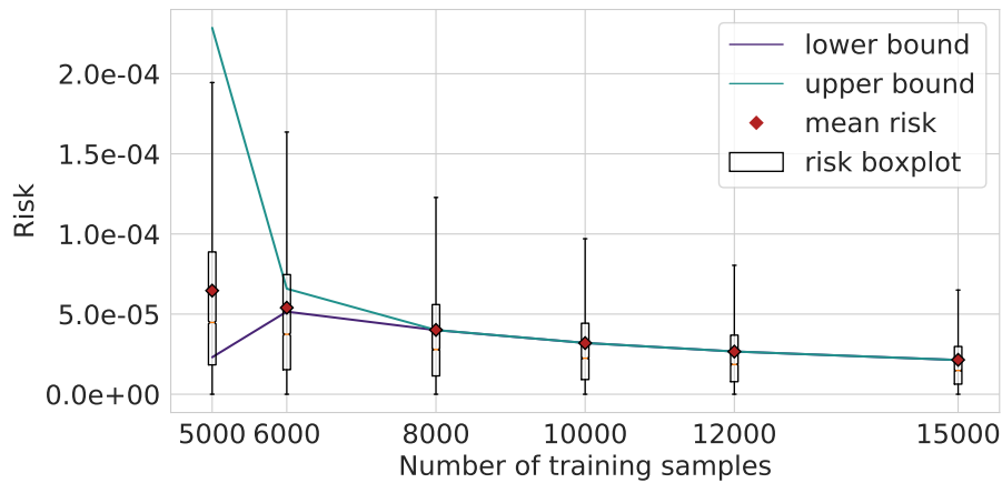
Figure S40. Illustration of the theoretical bounds for a shallow tree network of Proposition 4.2, for a chessboard with parameters k^* = 6 , N_B = 2^{k^* - 1} and p = 0.8 . The first-layer tree is of depth k = 6 . We draw a sample of size n (x-axis), and a single tree r_{k,0,n} is fitted for which the theoretical risk is evaluated. Each boxplot is built out of 20 000 repetitions. The outliers are not shown for the sake of presentation. Note that in such a case, the theoretical lower bound is constant and equal to the bias term.
