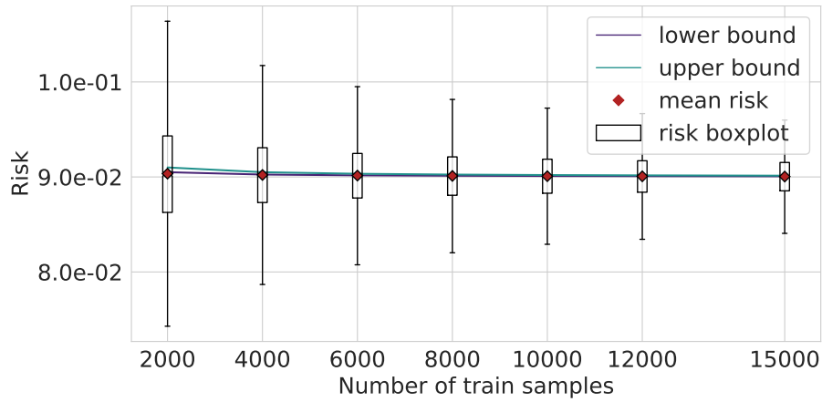
Figure S35. Illustration of the theoretical bounds for a single tree of Proposition 3 1. for a chessboard with parameters k^* = 4 , N_B = 2^{k^*-1} , and p = 0.8 . The single tree is of depth k = 2 . We draw a sample of size n (x-axis), and a single tree r_{k,0,n} is fitted for which the theoretical risk is evaluated. Each boxplot is built out of 20 000 repetitions. The outliers are not shown for the sake of presentation.
