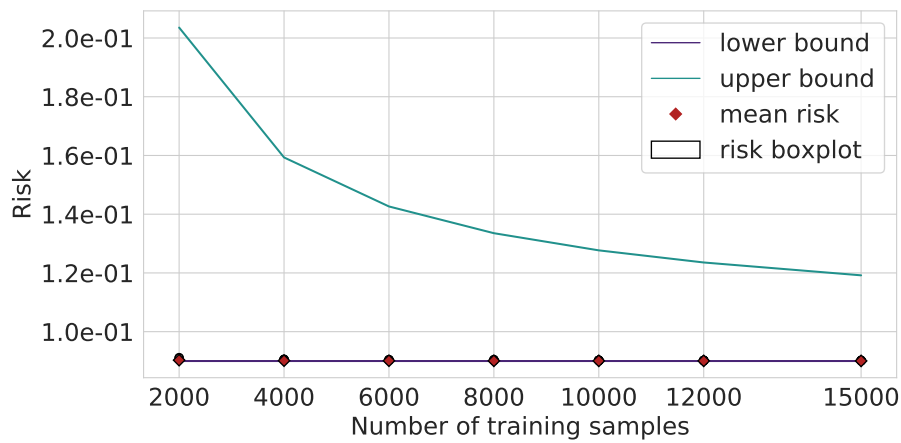
Figure S38. Illustration of the theoretical bounds for a shallow tree network of Proposition 3 2. for a chessboard with parameters k^* = 4 , N_B = 2^{k^*-1} and p = 0.8 . The first-layer tree is of depth k = 2 . We draw a sample of size n (x-axis), and a single tree r_{k,0,n} is fitted for which the theoretical risk is evaluated. Each boxplot is built out of 20 000 repetitions. The outliers are not shown for the sake of presentation. Note that in such a case, the theoretical lower bound is constant and equal to the bias term.
