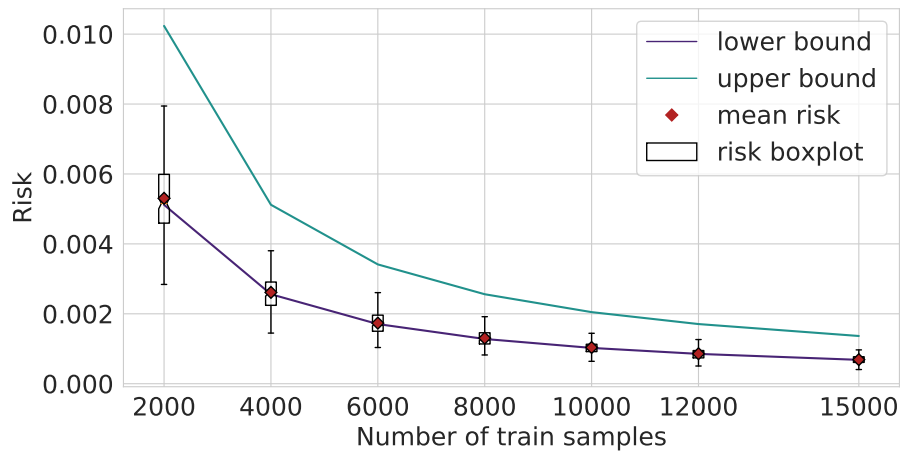
Figure S37. Illustration of the theoretical bounds for a single tree of Proposition 4 1. for a chessboard with parameters k^* = 4 , N_B = 2^{k^*-1} and p = 0.8 . The single tree is of depth k = 6 . We draw a sample of size n (x-axis), and a single tree r_{k,0,n} is fitted for which the theoretical risk is evaluated. Each boxplot is built out of 20 000 repetitions. The outliers are not shown for the sake of presentation.
