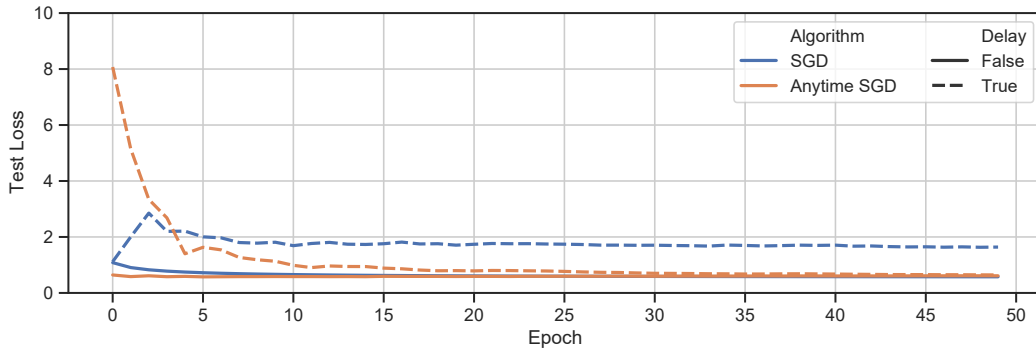
Figure 3. Expected excess loss as function of epochs when \tau_t = 500 , with learning rate optimized for each of the algorithms for zero delay regime.
