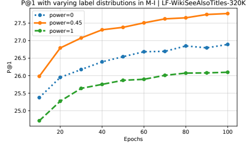
Figure 2: P@1 on LF-WikiSeeAlsoTitles-320K when label mini-batches are created in Module I using the label distribution raised to various powers. \text{power} = 0 gives the uniform distribution over labels whereas \text{power} = 1 recovers the (heavy-tailed) label distribution. Creating data-point mini-batches offers a label distribution similar to \text{power} = 1 .
