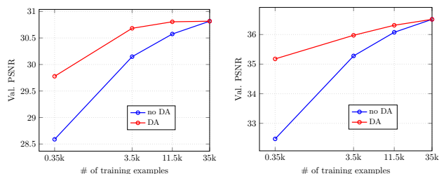
Figure 9. Single-coil (left) and multi-coil (right) validation PSNR vs. # of training images.
