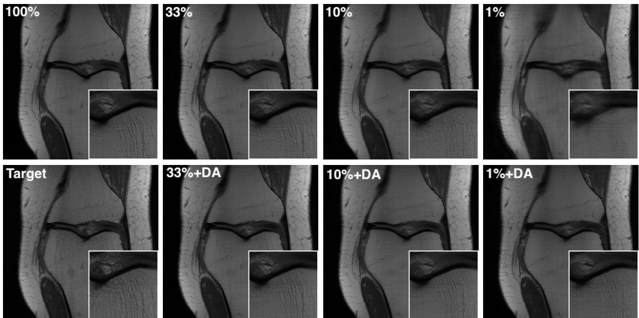
Figure 16. Visual comparison of fastMRI multi-coil reconstructions presented in Figure 6 extended with additional images corresponding to various amount of training data.
