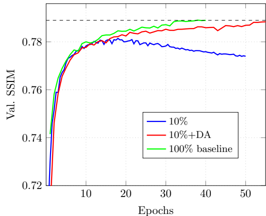
Figure 11. Results on the i-RIM network. We achieve SSIM comparable to the baseline with only 10% of the training data.
