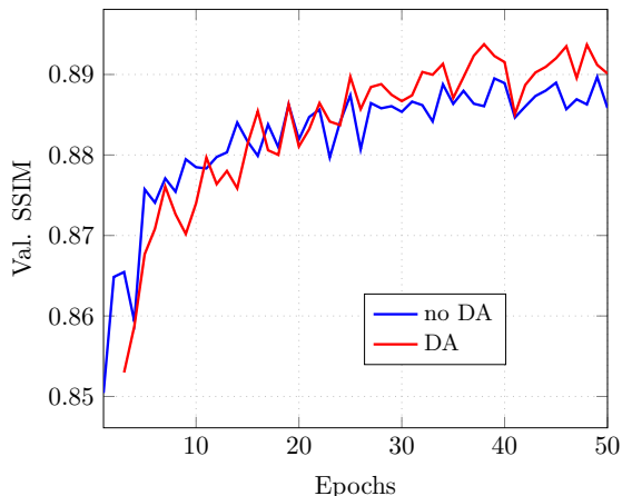
Figure 13. Val. performance of models trained on knee and evaluated on brain MRI.
