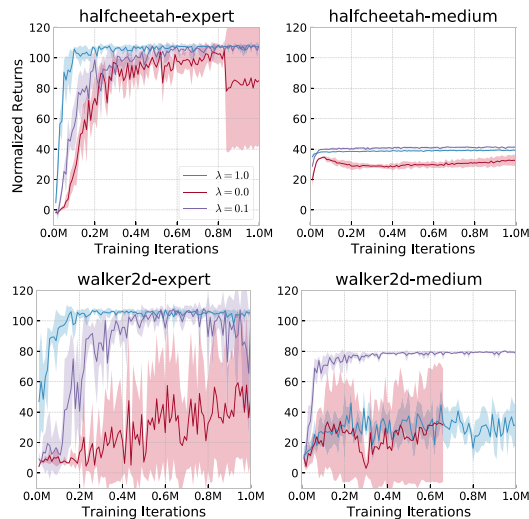
Figure 2. Performance of F-BRC for different values of the gradient penalty coefficient. A larger value, \lambda = 1 , over-constrains the learned policy to stay close to the behavior policy. This leads to more stable performance on expert datasets, where the behavior policy is near-optimal, but worse performance on medium datasets. Without the regularization ( \lambda = 0.0 ) Fisher-BRC collapses on most of these tasks; when the plot is cutoff, it means at least one of the seeds produced NaN values in training.
