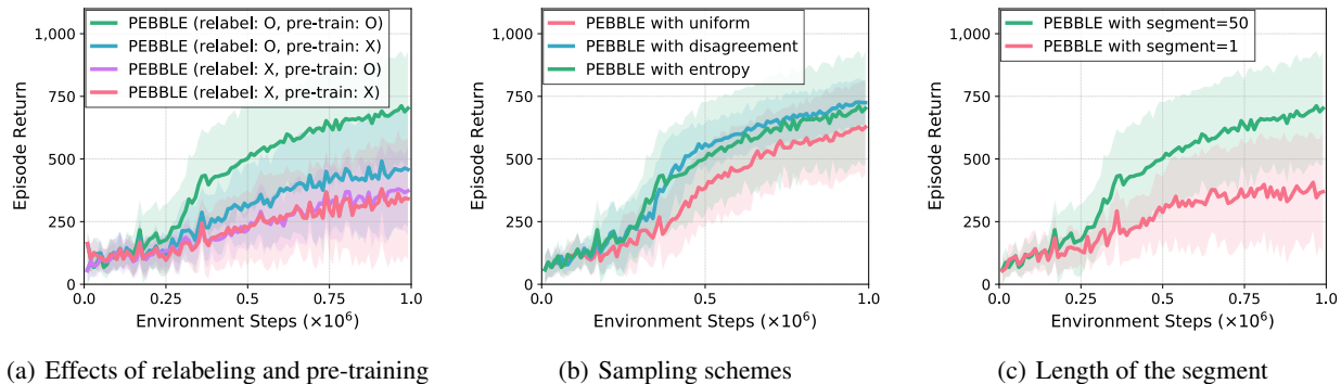
Figure 5. Ablation study on Quadruped-walk. (a) Contribution of each technique in PEBBLE, i.e., relabeling the replay buffer (relabel) and unsupervised pre-training (pre-train). (b) Effects of sampling schemes to select queries. (c) PEBBLE with varying the length of the segment. The results show the mean and standard deviation averaged over ten runs.
