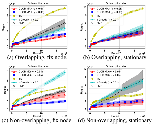
Figure 5. Regret for different online algorithms, when total budget B = 4000 .
