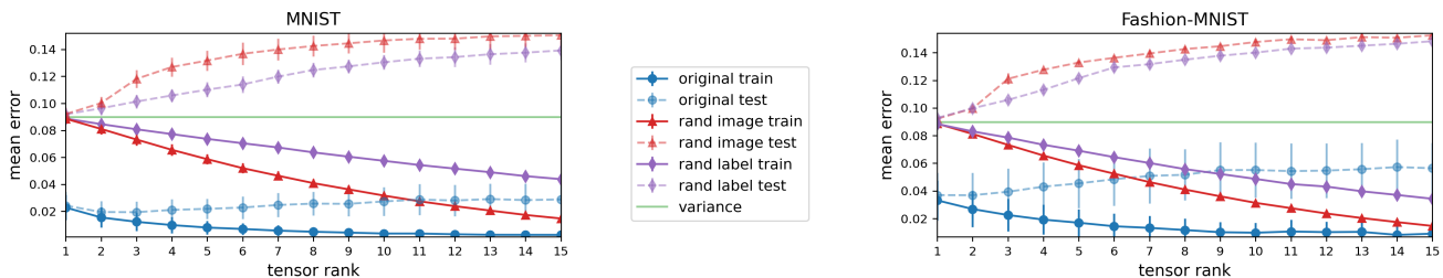
Figure 4: Evaluation of tensor rank as measure of complexity — standard datasets can be fit accurately with predictors of extremely low tensor rank (far beneath what is required by random datasets), suggesting it may capture the essence of natural data. Left and right plots show results of fitting MNIST and Fashion-MNIST datasets, respectively, with predictors of increasing tensor rank. Original datasets are compared against two random variants: one generated by replacing images with noise (“rand image”), and the other via shuffling labels (“rand label”). As described in the text (Subsection 5.2), for simplicity of presentation, each dataset was mapped into multiple (ten) one-vs-all prediction tasks (label 1 for active category, 0 for the rest), with fit measured via mean squared error. Separately for each one-vs-all prediction task and each value k \in \{1, \dots, 15\} for the tensor rank, we applied an approximate numerical method (see Subappendix B.2.2 for details) to find the predictor of tensor rank k (or less) with which the mean squared error over training examples is minimal. We report this mean squared error, as well as that obtained by the predictor on the test set (to mitigate impact of outliers, large squared errors over test samples were clipped — see Subappendix B.2.2 for details). Plots show, for each value of k , mean (as marker) and standard deviation (as error bar) of these errors taken over the different one-vs-all prediction tasks. Notice that the original datasets are fit accurately (low train error) by predictors of tensor rank as low as one, whereas random datasets are not (with tensor rank one, residuals of their fit are close to trivial, i.e. to the variance of the label). This suggests that tensor rank as a measure of complexity for predictors has potential to capture the essence of natural data. Notice also that, as expected, accurate fit with low tensor rank coincides with accurate prediction on test set, i.e. with generalization. For further details, as well as an experiment showing that linear predictors are incapable of accurately fitting the datasets, see Appendix B.
