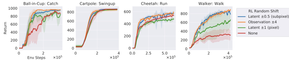
Figure 10. Even after pre-training encoders for DMControl using random shift, RL requires augmentation—our subpixel augmentation acts on the (compressed) latent image, permitting its use in the replay buffer.
