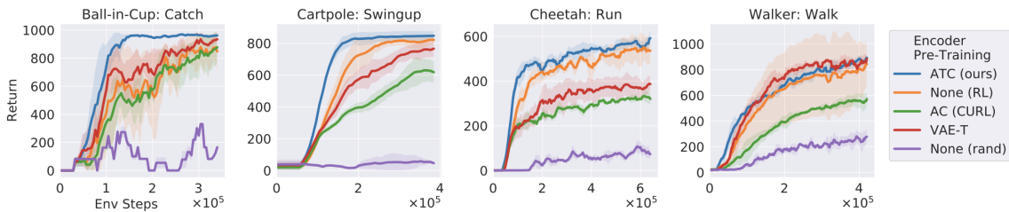
Figure 5. RL in DMControl, using encoders pre-trained on expert demonstrations using UL, with weights frozen—across all domains, ATC outperforms prior methods and the end-to-end RL reference. Each curve is a minimum of 4 random seeds.
