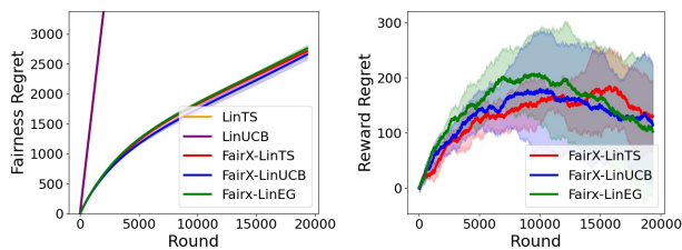
Figure 3. Fairness regret and reward regret of different linear bandit algorithms on the yeast dataset. ( c = 3 )
