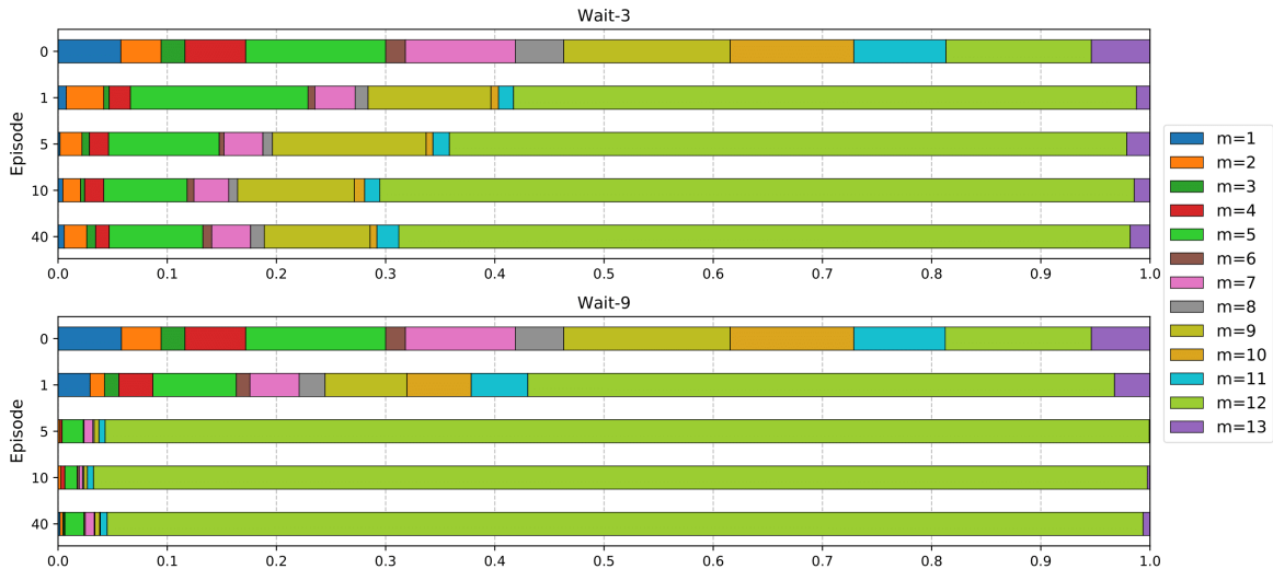
Figure 5: The distribution of wait-m tasks for wait-3 and wait-9 on En \rightarrow Zh dataset.
