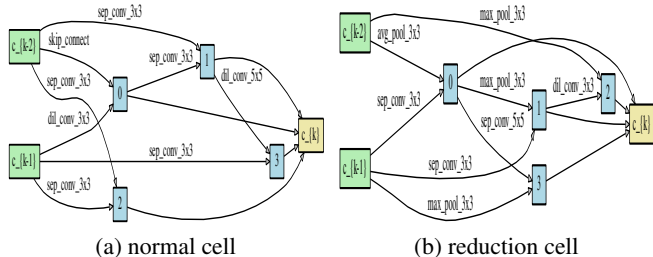
Figure 3. The best cells discovered by iDARTS on the DARTS search space.
