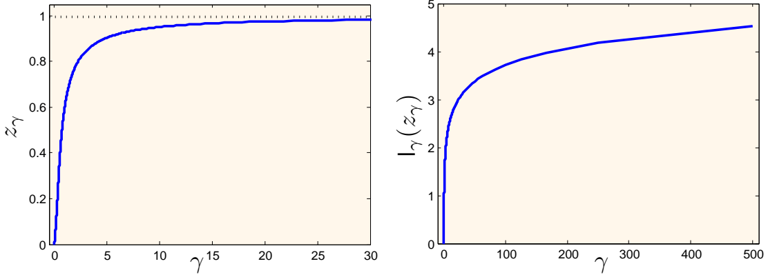
Figure 1: The plots of mappings \gamma \mapsto z_\gamma and \gamma \mapsto l_\gamma(z_\gamma) .
