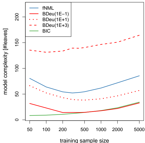
Figure 3: Complexity of the learned model structures w.r.t. the sample size and different structure scores: BIC, fnML, and BDeu (three different ESS values).
