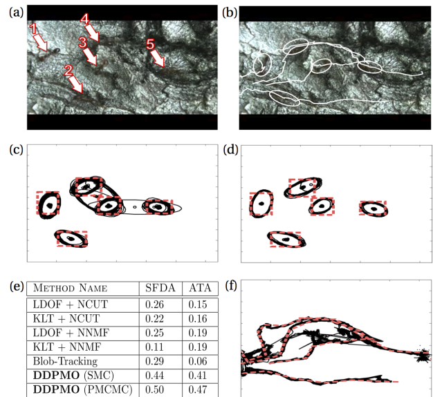
Figure 3: The ants in (a) are difficult to discern (positions labeled). We plot 100 samples from the inferred posterior over object parameters (using SMC (c) and PMCMC (d) with ground-truth bounding boxes overlaid (dashed). PMCMC proves to give more accurate object parameter samples. We also plot samples over object tracks (sequences of mean parameters) using PMCMC in (f), and its MAP sample in (b). We show the SFDA and ATA scores for all comparison methods in (e).
