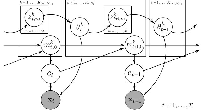
Figure 2: Graphical model of the dependent Dirichlet process mixture of objects (DDPMO). All observations at time t are denoted as \mathbf{x}_t and their assignments as c_t .
