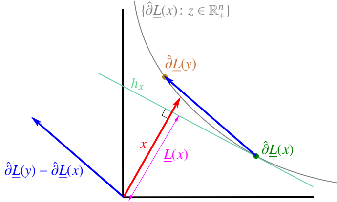
Figure 2: Geometrical interpretation of Bregman divergence \langle x, \hat{\partial}\underline{L}(y) - \hat{\partial}\underline{L}(x) \rangle when the concave function \underline{L} is 1-homogeneous and thus a concave support function of some convex set of positive type (whose lower left boundary is shown in grey).
