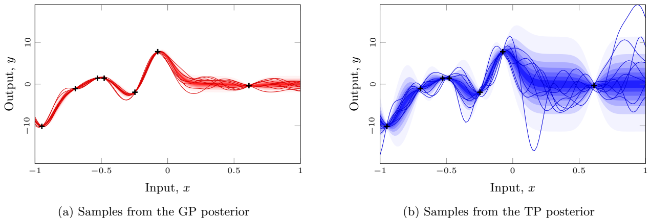
Figure 1: Demonstration of the added flexibility of the Student- t process in comparison with a Gaussian process with the same hyperparameter values for an exponentiated quadratic (squared exponential) covariance function. The shaded regions illustrate the 95% credible intervals.
