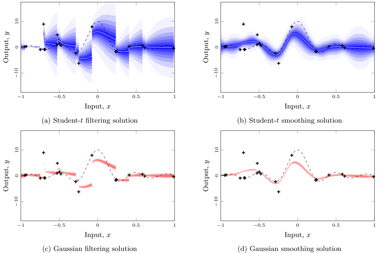
Figure 2: Comparison between the Student- t filtering and smoothing and the corresponding (Gaussian) Kalman filtering and Rauch–Tung–Striebel smoothing results for a set of measurements (+) of the scaled sinc function (---) featuring outliers. The shaded regions represent the 95% credible intervals. The hyperparameters were fixed to the same values for both the models.
