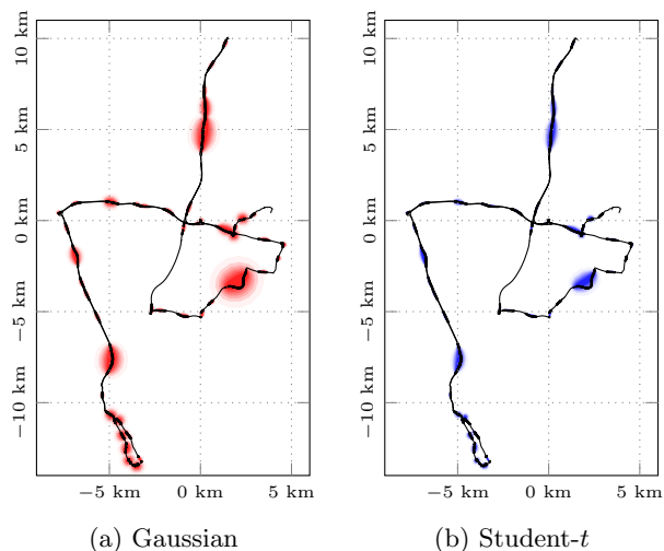
Figure 4: Interpolation of missing GPS observations by two-dimensional GP regression (Gaussian smoothing) and TP regression (Student- t smoothing). The unknown ground truth is shown by dots and the colored patches illustrate the credible intervals up to 95%.
