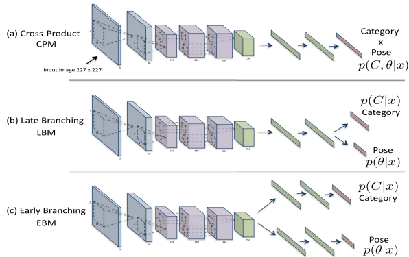
Figure 2. The studied models showing the joint loss layer in CPM, late branching in LBM and early branching in EBM. Blue layers correspond to layers with convolution, pooling and normalization. Violet colored layers correspond to layers with just convolution. Green layers correspond to fully-connected layers.
