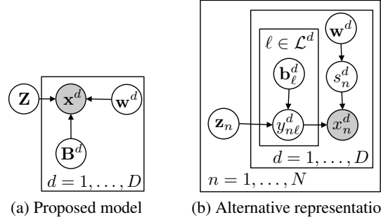
Figure 1. Model illustration.
