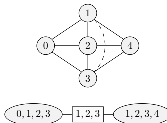
Figure 4: Example of clusters with mixture of interiors, boundaries and exteriors: (Top) the original graph and (Bottom) the junction tree, which introduces an edge from vertex 1 to vertex 3, so that 1 \not\perp 3 \mid 0, 2, 4 after tree decomposition. And for given interiors 1 and boundaries 0, 2, 4, there is an exterior 3 in the clusters.
