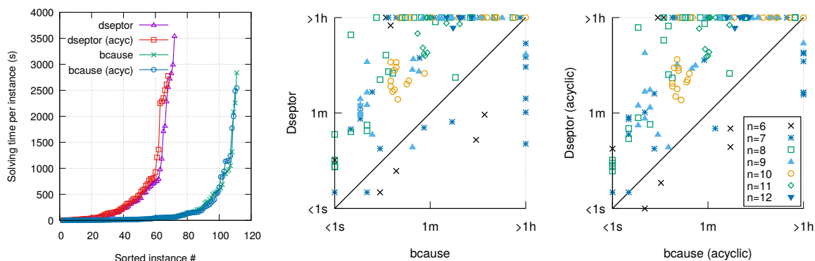
Figure 3: Running time performance comparison: bcause v dseptor.
