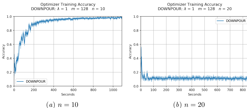
Figure 2: DOWNPOUR divergence due to number ( n = 20 ) of asynchronous workers in the optimization process Mitliagkas et al. (2016) for this particular problem, and not dealing with parameter staleness in a more intelligent way. Lowering the number workers ( n = 10 ) causes the central variable to converge.
