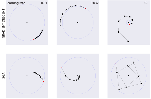
Figure 3. SGA allows faster and more robust convergence to stable fixed points. Note the scale of top-right panel differs from rest.
