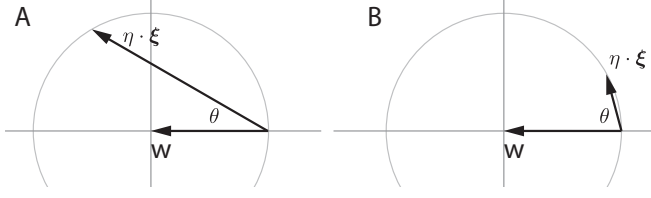
Figure 6. Alignment and learning rates. The larger \cos \theta , the larger the learning rate \eta that can be applied to unit vector \xi without \mathbf{w} + \eta \cdot \xi leaving the unit circle.
