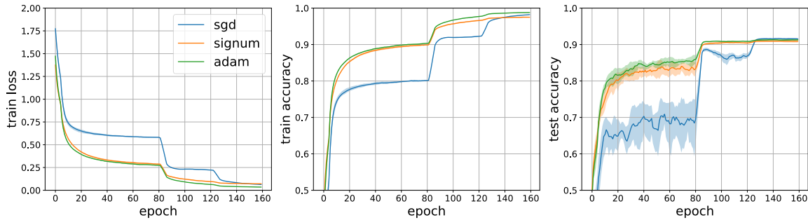
Figure A.3. CIFAR-10 results using SIGNUM to train a Resnet-20 model. Top: validation accuracies from a hyperparameter sweep on a separate validation set carved out from the training set. We used this to tune initial learning rate, weight decay and momentum for all algorithms. All other hyperparameter settings were chosen as in (He et al., 2016a) as found favourable for SGD. The hyperparameter sweep for other values of momentum is plotted in Figure A.4 of the supplementary. Bottom: there is little difference between the final test set performance of the algorithms. SIGNUM closely resembles ADAM in all of these plots.
