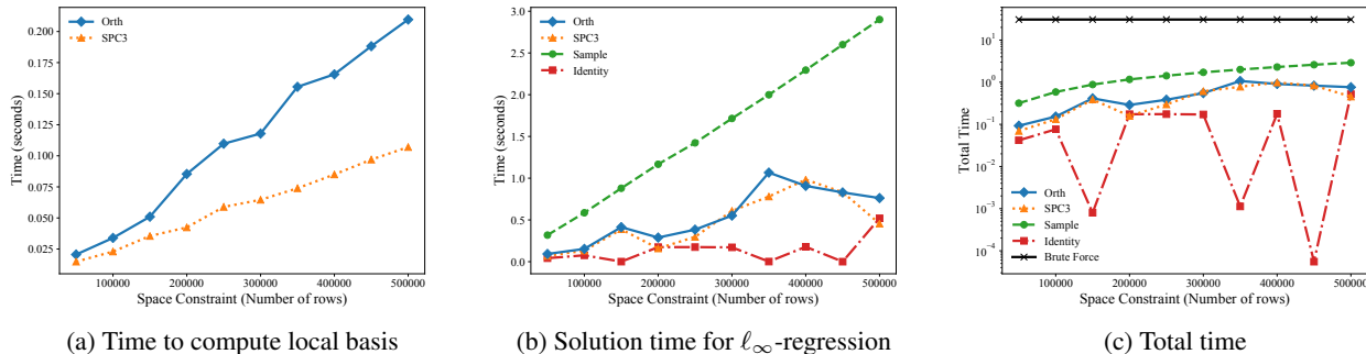
Figure 3: Computation Times compared to summary size
