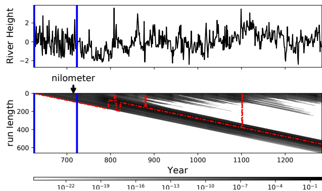
Figure 5. Results for Nile data: Panel 1: Nile data with structural change at 715. Panel 2: Both run-length distribution (grayscale with dashed maximum) and MAP segmentation detect the change.
