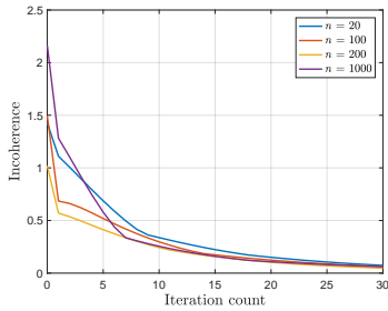
Figure 3. The incoherence measure \frac{\max_{1 \leq j \leq m} |\mathbf{a}_j^\top(\mathbf{x}^t - \mathbf{x}^h)|}{\sqrt{\log n} \|\mathbf{x}^h\|_2} of the gradient iterates vs. iteration count for the phase retrieval problem. The results are shown for n \in \{20, 100, 200, 1000\} and m = 10n , with the step size taken to be \eta_t = 0.1 . The problem instances are generated in the same way as in Figure 1.
