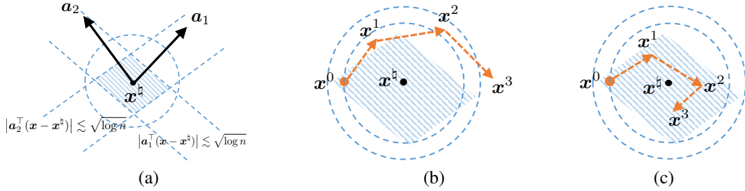
Figure 2. (a) The shaded region is an illustration of the incoherence region, which satisfies |\mathbf{a}_j^\top(\mathbf{x} - \mathbf{x}^h)| \lesssim \sqrt{\log n} for all points \mathbf{x} in the region. (b) When \mathbf{x}^0 resides in the desired region, we know that \mathbf{x}^1 remains within the \ell_2 ball but might fall out of the incoherence region (the shaded region). Once \mathbf{x}^1 leaves the incoherence region, we lose control and may overshoot. (c) Our theory reveals that with high probability, all iterates will stay within the incoherence region, enabling fast convergence.
