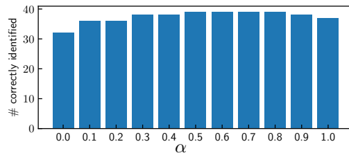
Figure 4. Model selection: trade-off between sparsity and validation error, see Eq. (9) with \beta = 1 - \alpha , evaluated empirically in terms of the number of correctly identified equations on all the datasets considered in Section 4. We choose the canonical \alpha = 0.5 as the differences between 0.3 and 0.9 are not significant.
