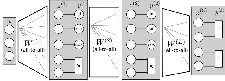
Figure 1. Network architecture of the proposed improved Equation Learner \text{EQL}^{\ddagger} for 3 layers ( L = 3 ) and one neuron per type ( u = 3, v = 1 ). The new division operations are places in the final layer, see Martius & Lampert (2016) for the original model.
