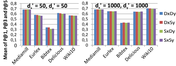
Figure 2. Comparison of the four combinations for node diversity for two values of (d'_x, d'_y) for a fifty tree forest.
