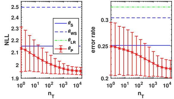
(a) n_S = 8, \mu_1 = -\mu_0 = 0.5
