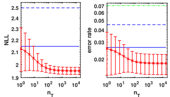
(b) n_S = 8, \mu_1 = -\mu_0 = 2
