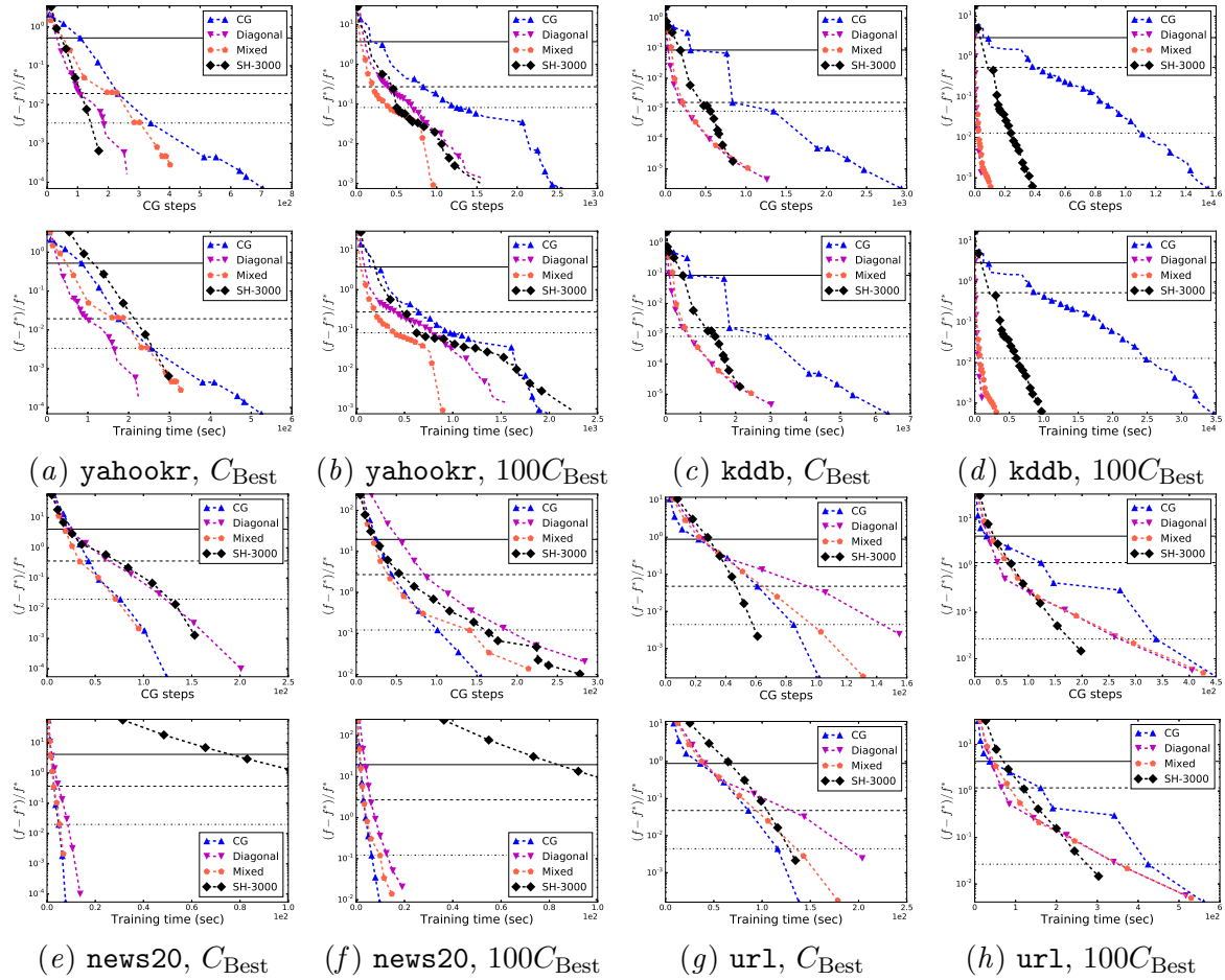
Figure 2: Convergence of using different preconditioners. We present the results of using C = C_{\text{Best}} and C = 100C_{\text{Best}} . For the same data set and under the same C value, the x -axis of the upper figure is the cumulative number of CG steps and the x -axis of the lower one is the running time. We align curves of the approach CG in upper and lower figures for an easy comparison. Other settings are the same as those in Figure 1.
