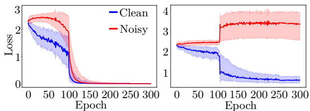
Figure 1. Cross-entropy loss on CIFAR-10 under 80% label noise for clean and noisy samples. Left: training with cross-entropy loss results in fitting the noisy labels. Right: using our proposed objective prevents fitting label noise while also learning from the noisy samples. The heavy lines represent the median losses and the shaded areas are the interquartile ranges.
