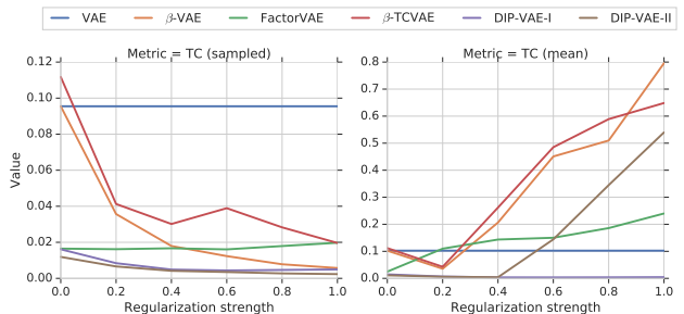
Figure 1. Total correlation based on a fitted Gaussian of the sampled (left) and the mean representation (right) plotted against regularization strength for Color-dSprites and approaches (except AnnealedVAE). The total correlation of the sampled representation decreases while the total correlation of the mean representation increases as the regularization strength is increased.
