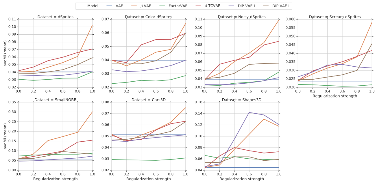
Figure 28. The average mutual information of the dimensions of the mean representation generally increase.
