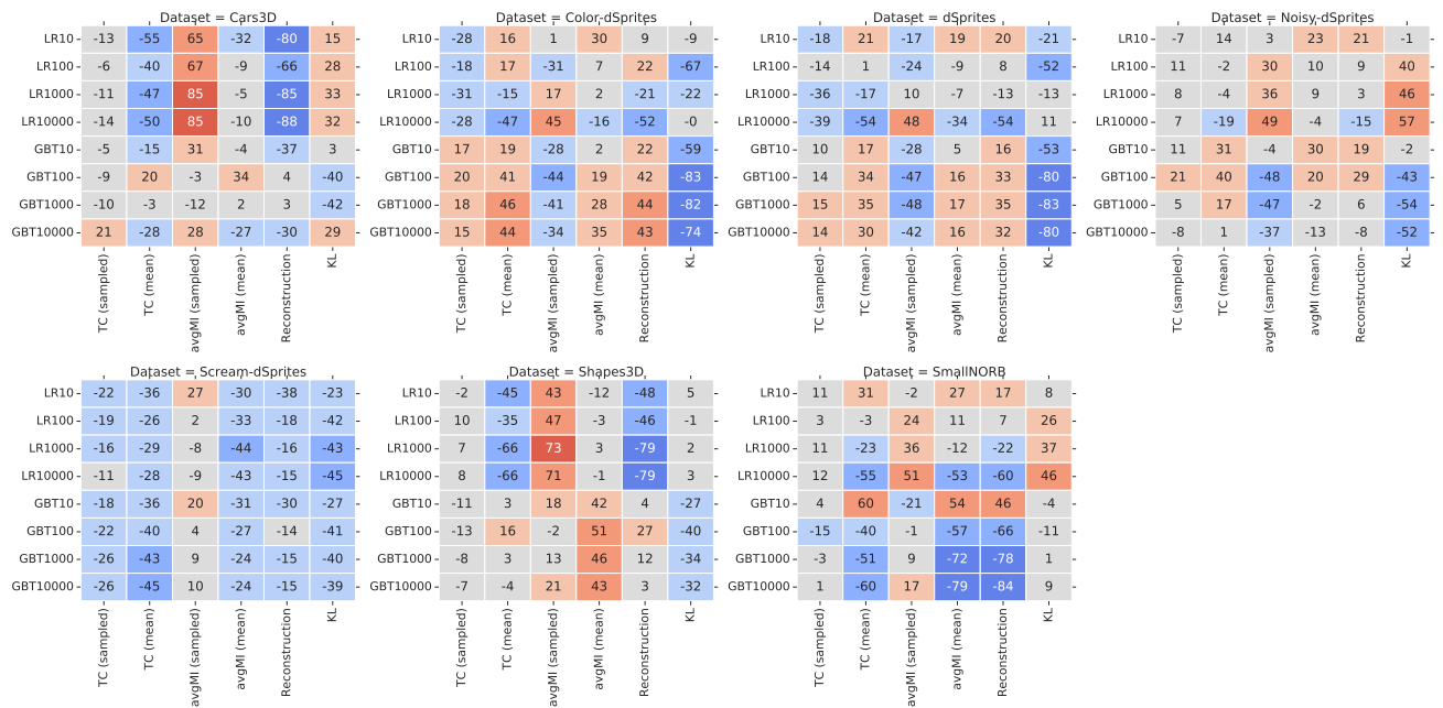
Figure 24. Rank correlation between unsupervised scores and downstream performance.
