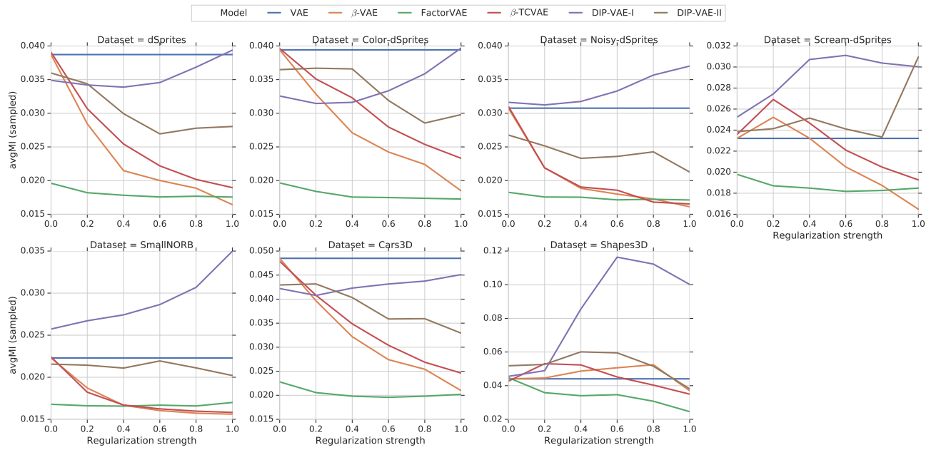
Figure 27. The average mutual information of the dimensions of the sampled representation generally decrease except for DIP-VAE-I.
