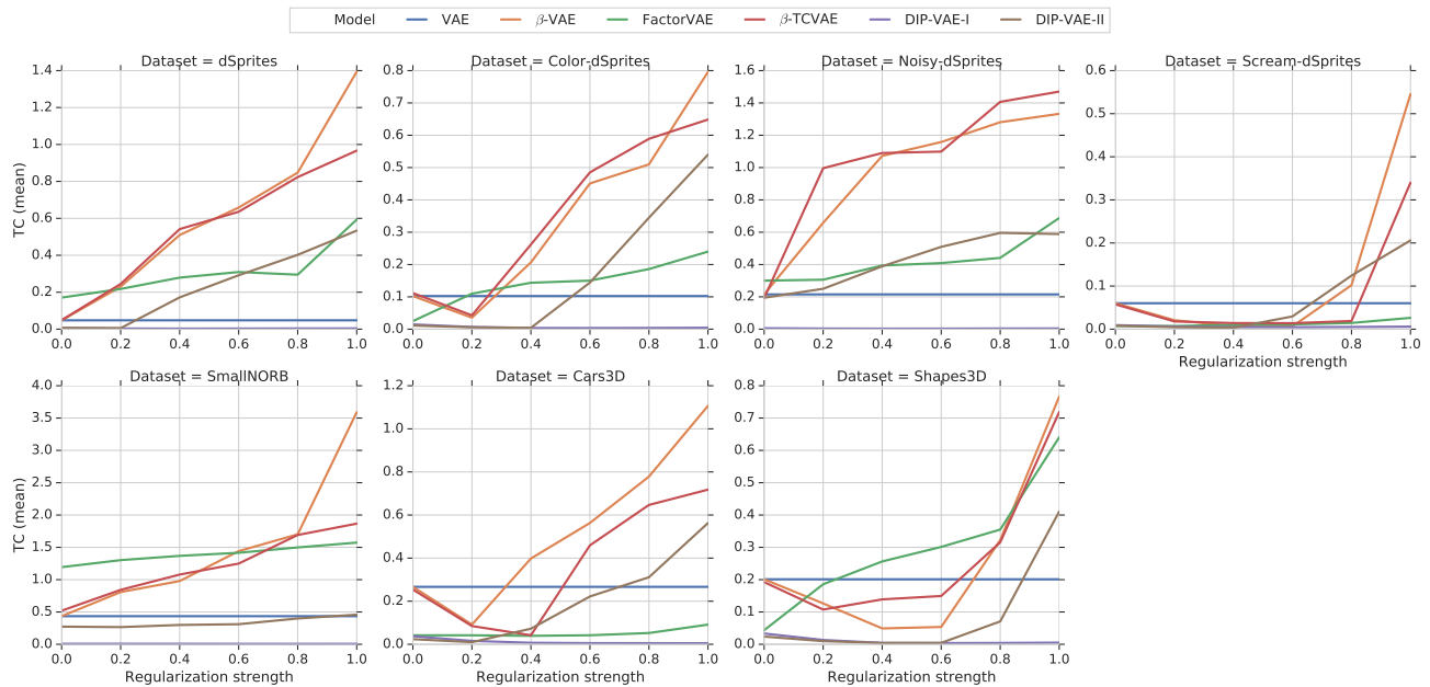
Figure 9. Total correlation of mean representation plotted against regularization strength for different data sets and approaches (except AnnealedVAE). The total correlation of the mean representation does not necessarily decrease as the regularization strength is increased.
