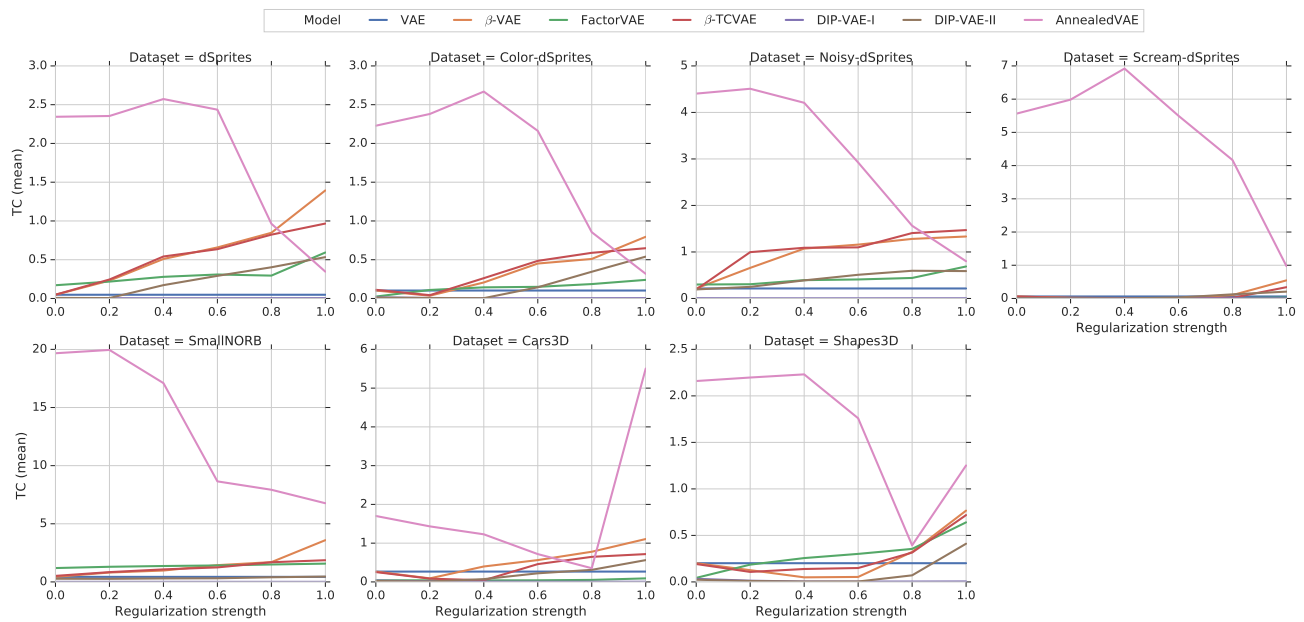
Figure 26. Total correlation of mean representation plotted against regularization strength for different data sets and approaches (including AnnealedVAE).
