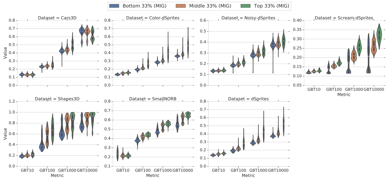
Figure 23. Downstream performance for three groups with increasing MIG scores.
