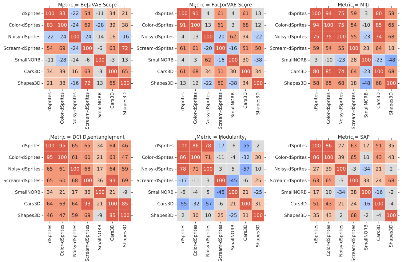
Figure 17. Rank-correlation of different disentanglement metrics across different data sets. Good hyperparameters only seem to transfer between dSprites and Color-dSprites but not in between the other data sets.
