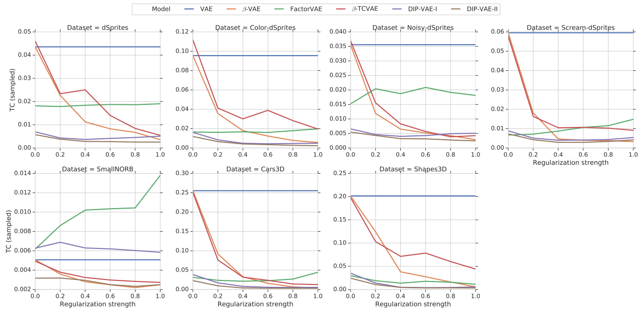
Figure 8. Total correlation of sampled representation plotted against regularization strength for different data sets and approaches (except AnnealedVAE). The total correlation of the sampled representation decreases as the regularization strength is increased.
