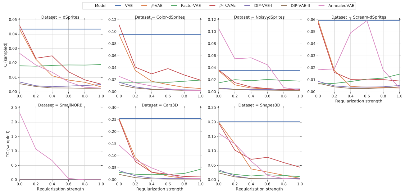
Figure 25. Total correlation of sampled representation plotted against regularization strength for different data sets and approaches (including AnnealedVAE).
