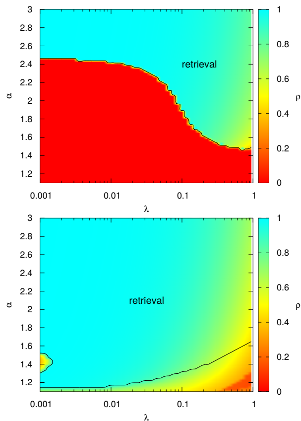
Figure 2. Phase diagrams corresponding to the SE asymptotic analysis of GAMP (top) and GASP (bottom). The color maps indicate the overlap \rho reached at convergence in the presence of an L_2 regularizer of intensity \lambda .
