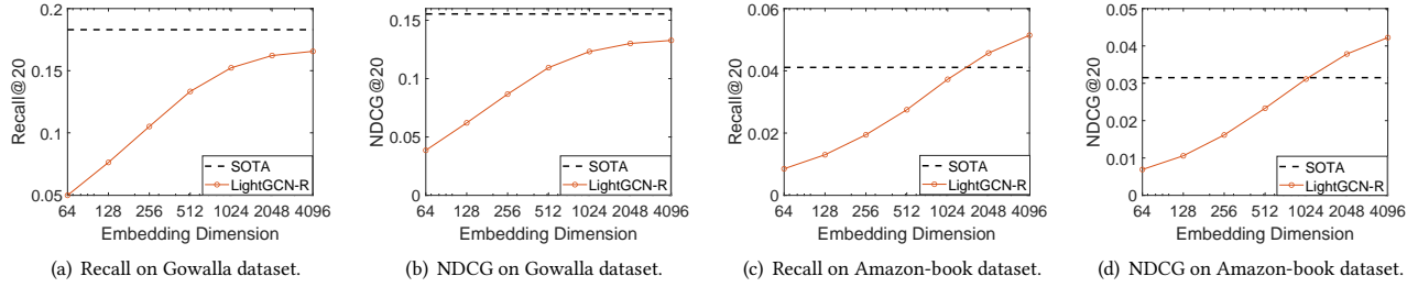
Figure 1: Performance of untrained LightGCN versus SOTA, where the SOTA line is LightGCN’s performance reported in [13] and LightGCN-R denotes the untrained LightGCN with different embedding dimensions.
