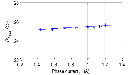
Fig. 12. Locked-rotor resistance obtained from the six-phase test.
