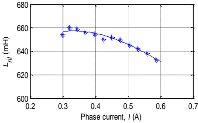
Fig. 10. No-load inductance obtained from the six-phase test.
