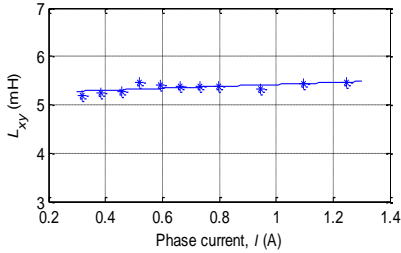
Fig. 13. Inductance obtained from the x - y plane excitation.
