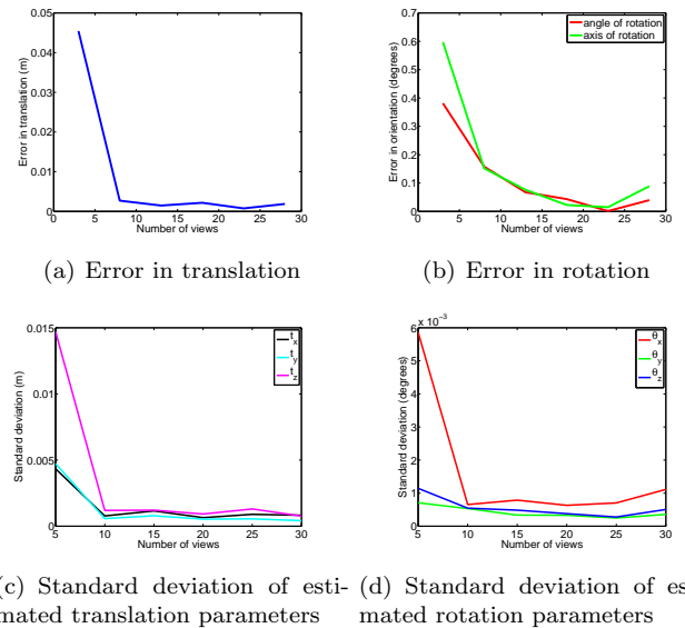
Fig. 7. Simulation results: Error in estimation decreases as number of views of target plane increases. Area of plane = 1m²
