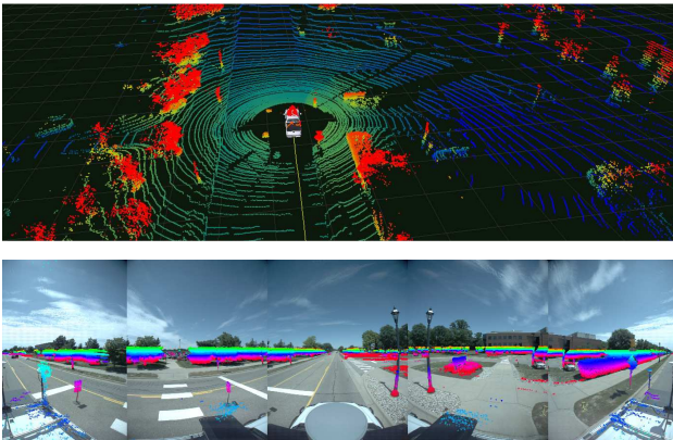
Fig. 10. The top panel is a perspective view of the Velodyne lidar range data, color-coded by height above the estimated ground plane. The bottom panel shows the above-ground-plane range data projected into the corresponding image from the Ladybug cameras.
