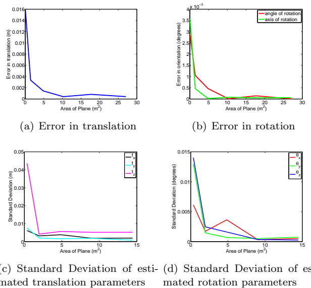
Fig. 6. Simulation results: Error in estimation decreases as area of target plane increases. Number of views = 10
