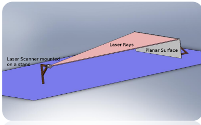
Fig. 2. Depiction of the manual calibration technique used by the manufacturers to estimate the range offset corresponding to each laser.
