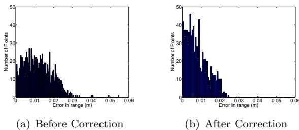
Fig. 4. Histogram of error in range of points falling on the plane. The error is the perpendicular distance of the inlier points from the estimated plane. The plane equation and the inliers are estimated using RANSAC.
