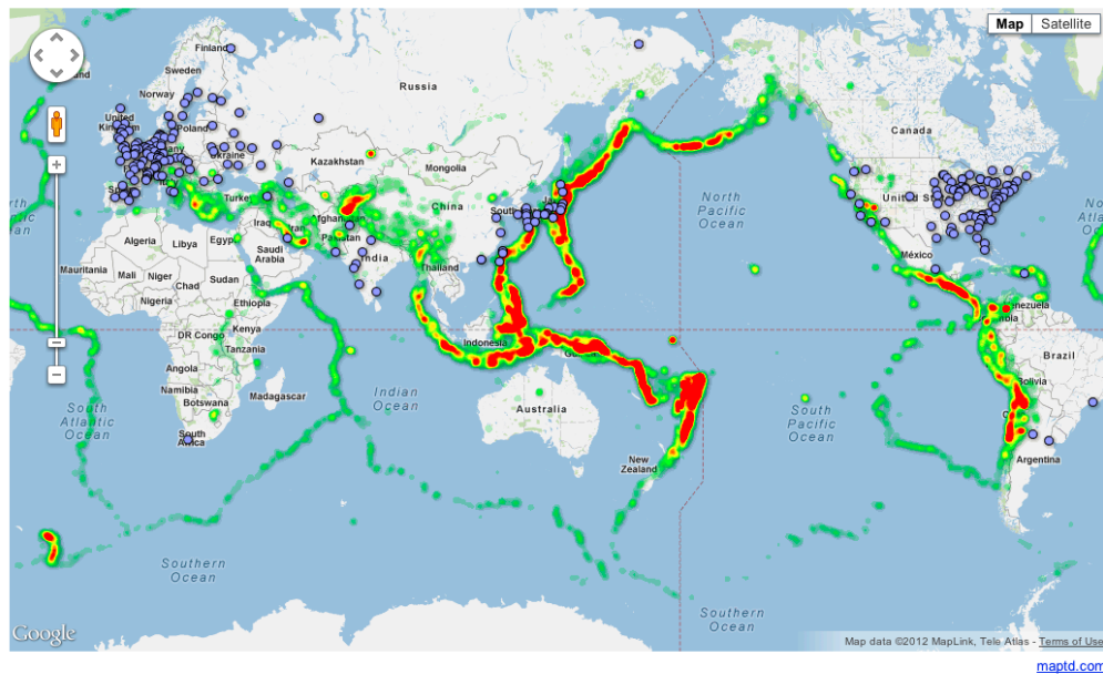
Global earthquake activity since 1973 and nuclear power plant locations
