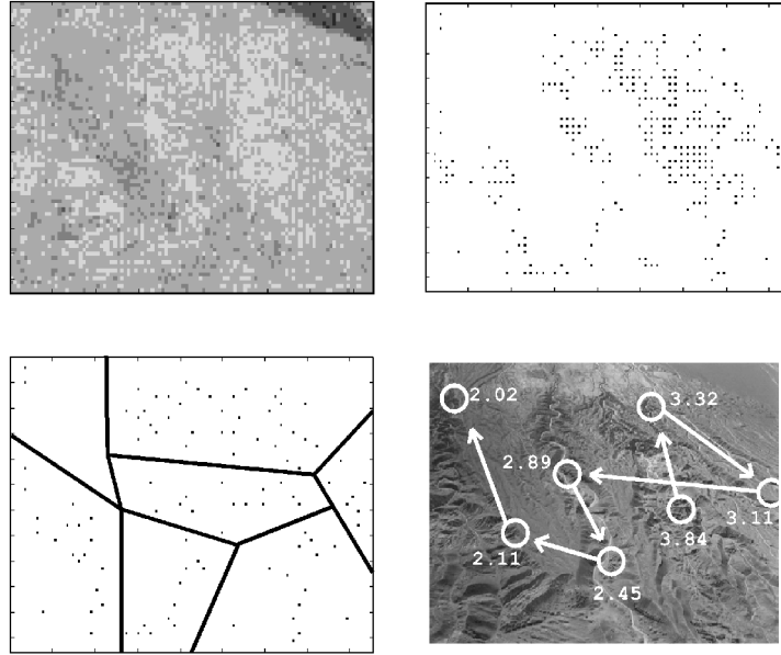
Fig. 4. Clustering Procedure: To completion—Algorithm \mathcal{N} , entropy, is applied to a Chilean desert photo (upper left). The initial set of local maxima (upper right) is then clustered using the defined iterative procedure (lower left: partway through the process). The final ordering, superimposed on the original image, is shown in the lower right panel; the maximum-valued locus for each cluster is inserted in the figure.
